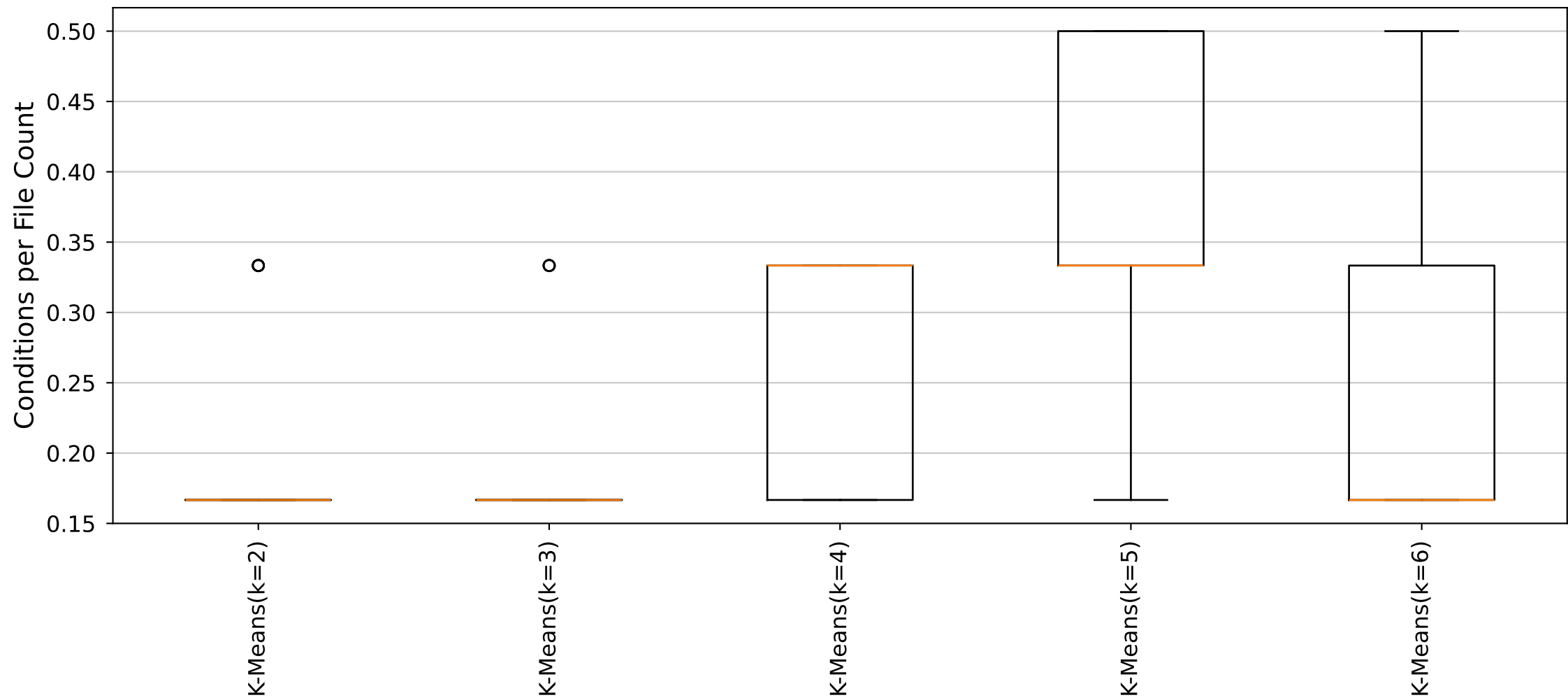
YARA Rules Conditions per File Count Distribution (Cluster19_Size6 dataset)
